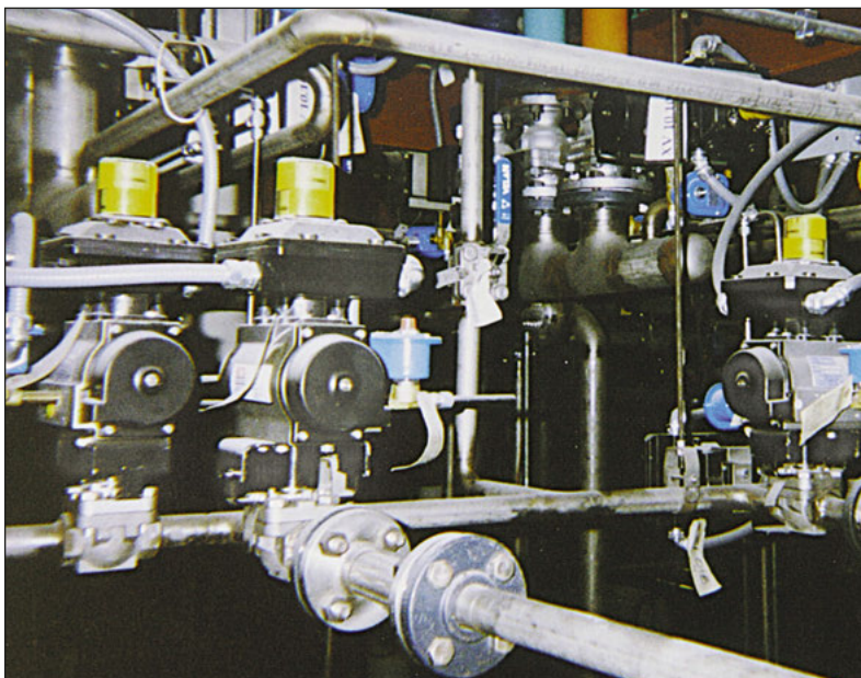
Top-entry ball valve installation.
