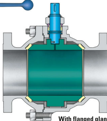
With flanged gland
